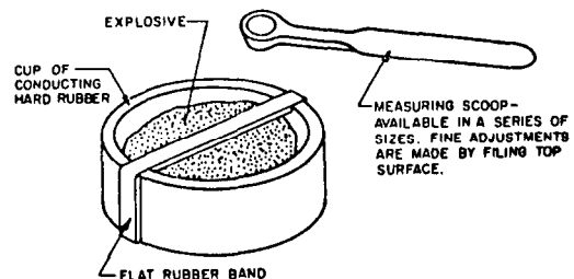
Fig 1 Scoop Loading
